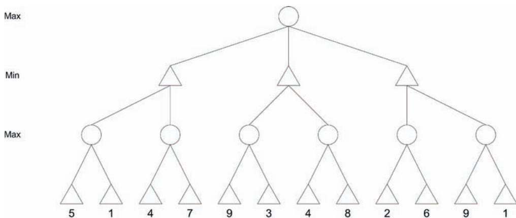
FIGURE 4.24: Sample game tree for minimax search.
