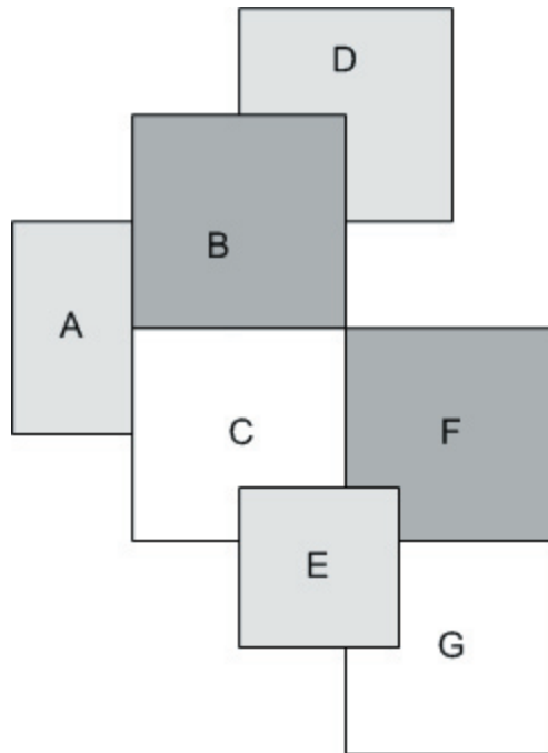
FIGURE 3.16: Result of Graph Coloring from Listing 3.17.
