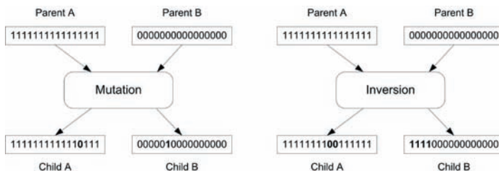
FIGURE 7.10: Illustrating the mutation and inversion genetic operators.
