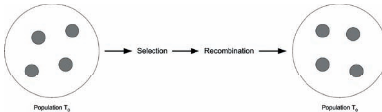
FIGURE 7.5: Fundamental process of population-based evolutionary algorithms.
