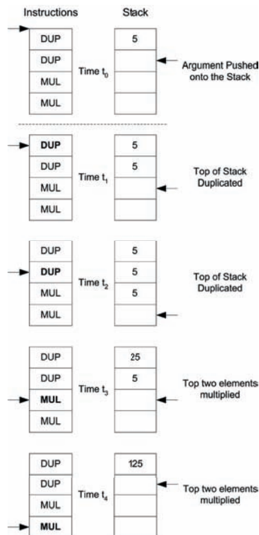
FIGURE 7.17: Example instruction sequence and stack for the 'cube' program.
