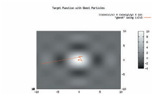
FIGURE 7.26: Global best particle fitness showing quick convergence and then solution tuning with slowing velocities.
