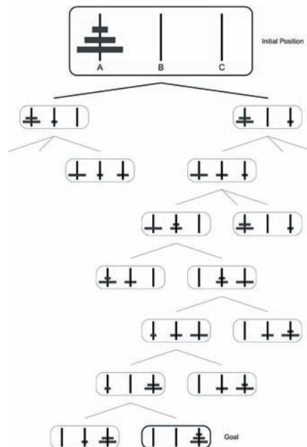
FIGURE 2.3: A search space for the “Tower of Hanoi” puzzle.
