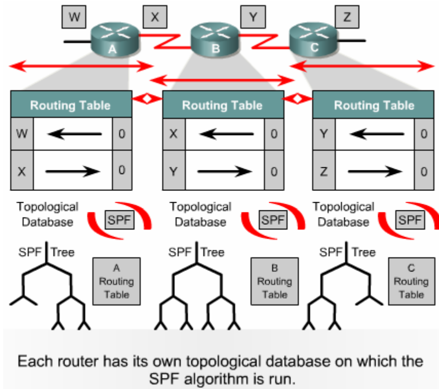
Gambar 6.23 jaringan link-state discovery
