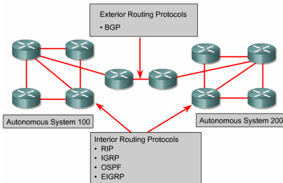
Gambar 6.30 protokol-protokol routing IP
