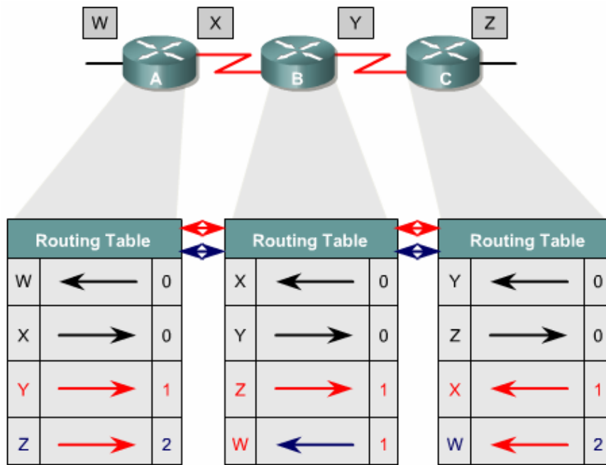
Gambar 6.19 jaringan distance vector discovery
