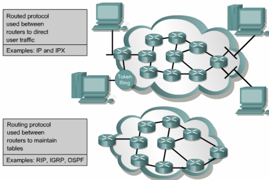
Gambar 6.14 Routed vs Routing Protokol
